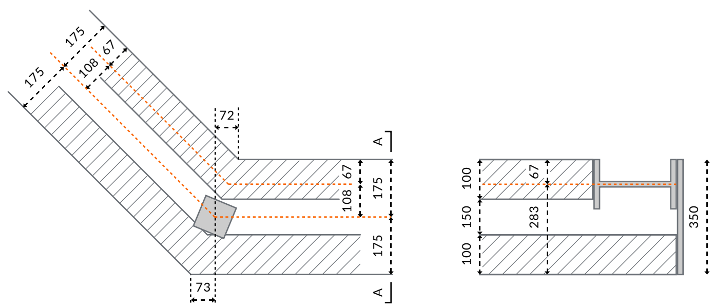
POST LOCATION FOR 350 WIDE WALL
