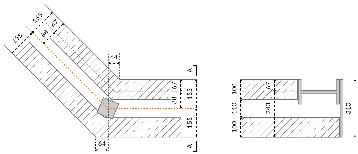
POST LOCATION FOR 310 WIDE WALL
