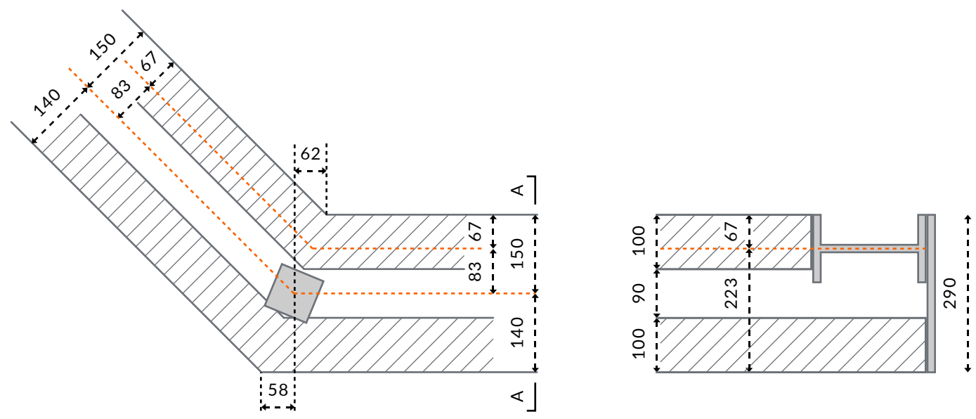
POST LOCATION FOR 290 WIDE WALL
