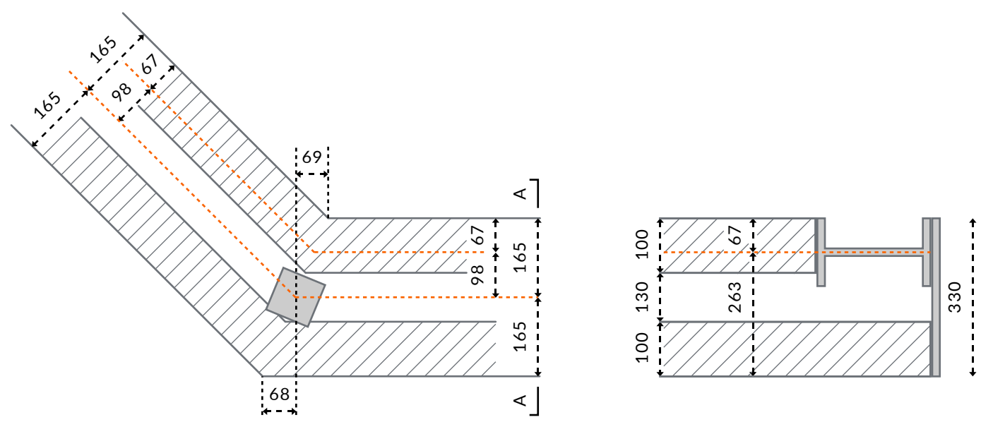
POST LOCATION FOR 330 WIDE WALL
