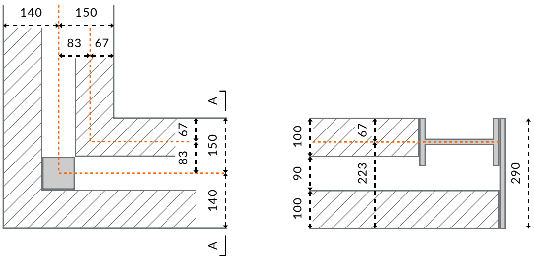
POST LOCATION FOR 290 WIDE WALL
