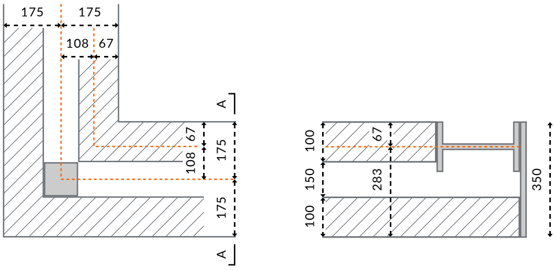
POST LOCATION FOR 350 WIDE WALL
