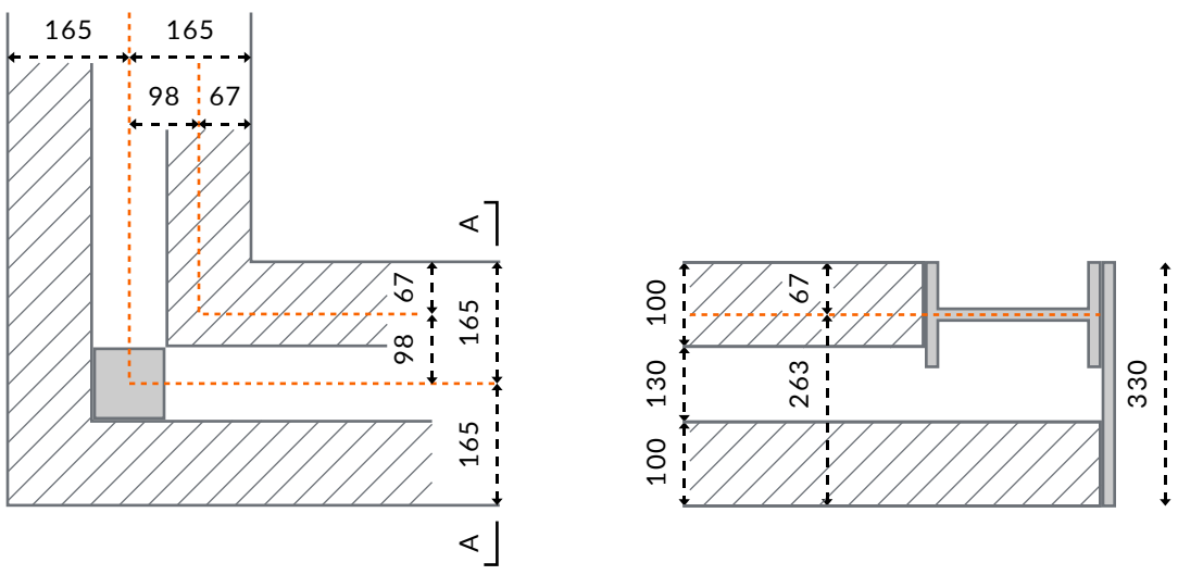
POST LOCATION FOR 330 WIDE WALL
