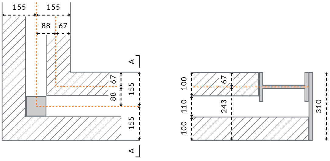
POST LOCATION FOR 310 WIDE WALL
