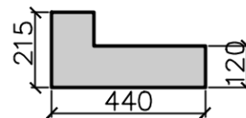
Alt for render using MA55 Quoins (31kg)
