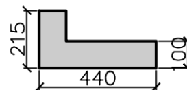
Quoin Stack using MA05 Quoins (26kg)
